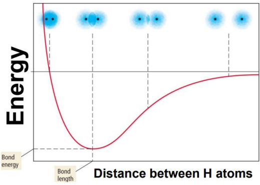
Interaction Energy of Two Hydrogen Atoms
